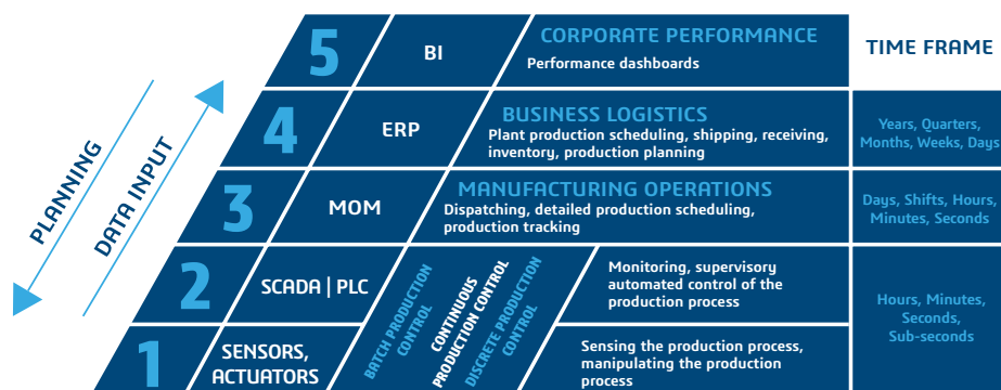
ISA-95 Enterprise Systems Hierarchy Representation.
